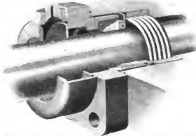
Fig. 1019. Piston Rod Packing with Glands vibrating Cup. U. S. Metallic Packing Co.
